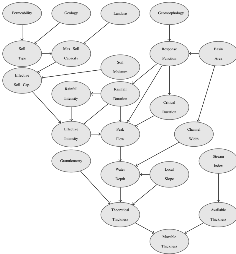
Figure 7: A credal network for environmental risk analysis.
