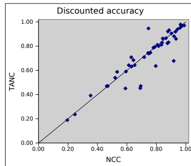
Figure 16: Discounted accuracy of TANC and NCC.
