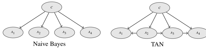
Figure 14: TAN can model dependencies between features, unlike naive Bayes.
