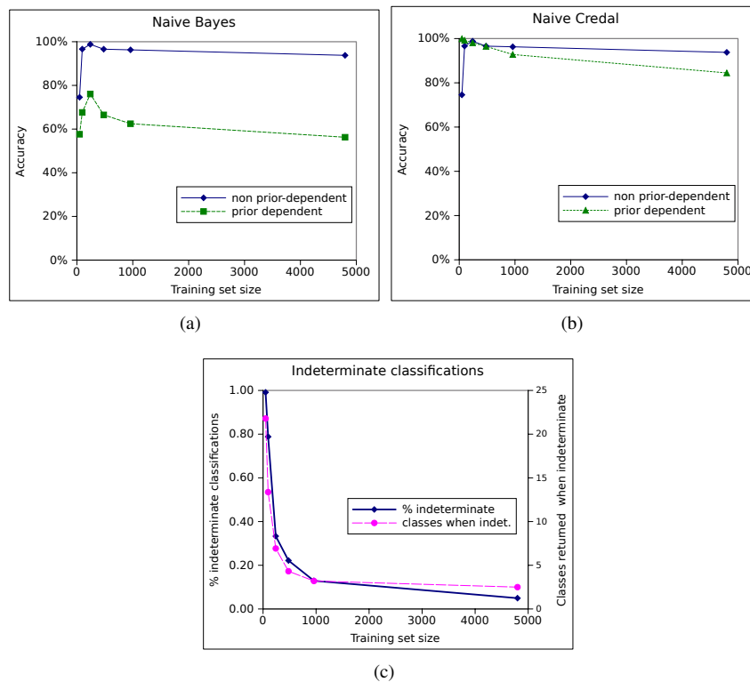
Figure 13: Experiments with varying sizes of the training set. Plots (a) and (b) show the accuracy of NBC and NCC on instances which are prior dependent (dashed) and non prior-dependent (solid); plot (c) shows the percentage of indeterminate classifications (solid) and the average number of classes returned by NCC when indeterminate (dashed).
