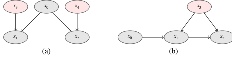
Figure 4: Modelling non-separately specific conditional credal sets with control nodes (in pink).
