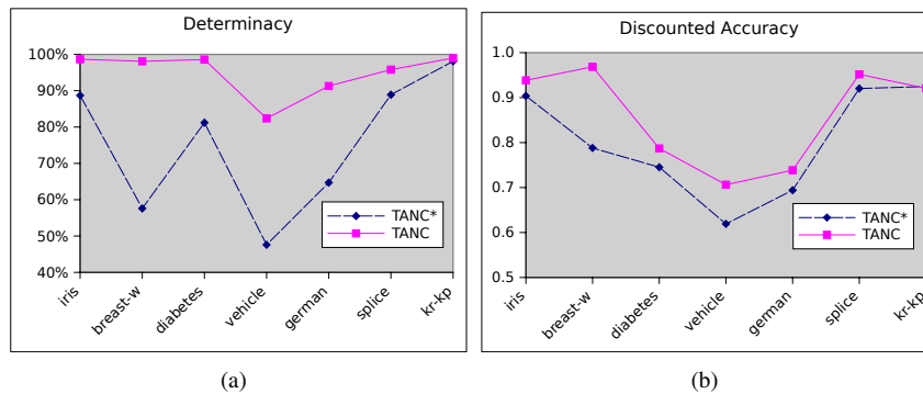
Figure 15: Comparison of TANC* and TANC. Plot (a) shows the determinacy (% of determinate classifications) of the classifiers on different data sets, while plot (b) shows their discounted accuracy.
