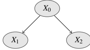
Figure 2: A credal network over three binary variables. Concerning quantification, we set \text{ext}[K(X_0)] = \{[.2, .8]^T, [.5, .5]^T\} , \text{ext}[K(X_1|x_0)] = \{[.3, .7]^T, [.4, .6]^T\} , \text{ext}[K(X_1|\neg x_0)] = \{[.1, .9]^T, [.2, .8]^T\} , \text{ext}[K(X_2|x_0)] = \{[.5, .5]^T, [.6, .4]^T\} , \text{ext}[K(X_2|\neg x_0)] = \{[.7, .3]^T, [.8, .2]^T\} .
