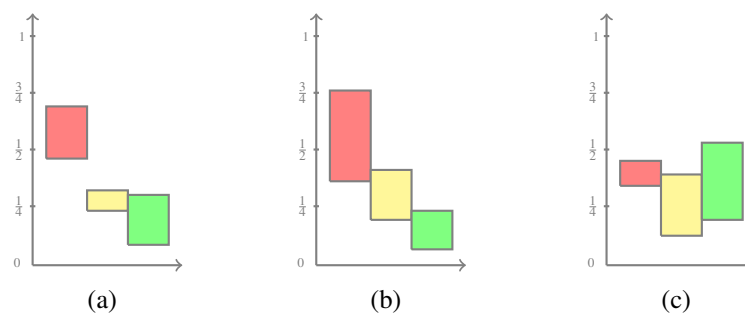
Figure 10: Posterior probability intervals for the three level of risk (colors red, yellow and green correspond respectively to high, medium and low risk).
