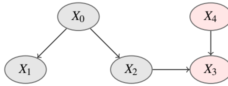
Figure 5: Modelling non-missing-at-random observation of X_2 in credal network.
