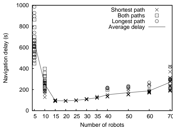
Fig. 11. Navigation delay versus number of robots in the scenario of figure 10. The choice of path in each test is shown by the point symbols.
