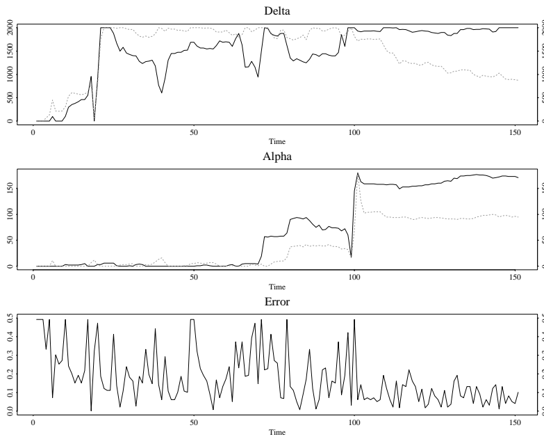
Figure 8: A team of two heterogeneous Ibots: Ibot 1 (dashed line) moves 4 times faster than Ibot 2 (solid line), which is blind. Time evolution of \delta^i_{prog} s (first plot), of \alpha^i_{prog} s (second plot), and of the error E (third plot).
