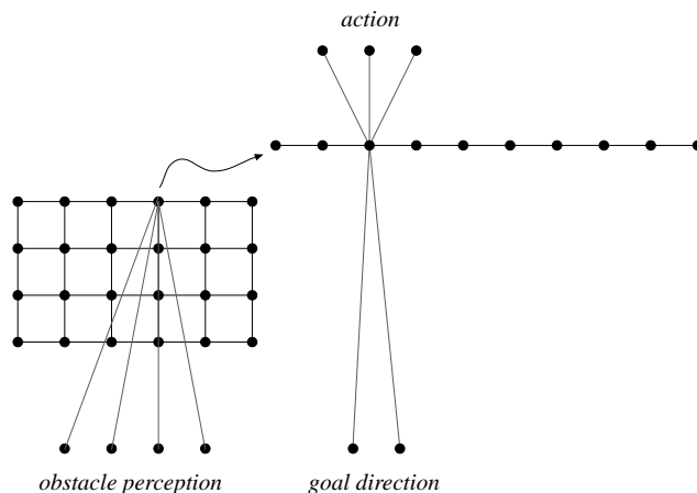
Figure 24: The HEKM network architecture.
