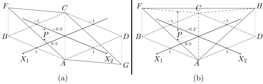
Fig. 1. Random quantities and sets of coherent previsions in Example 1.
